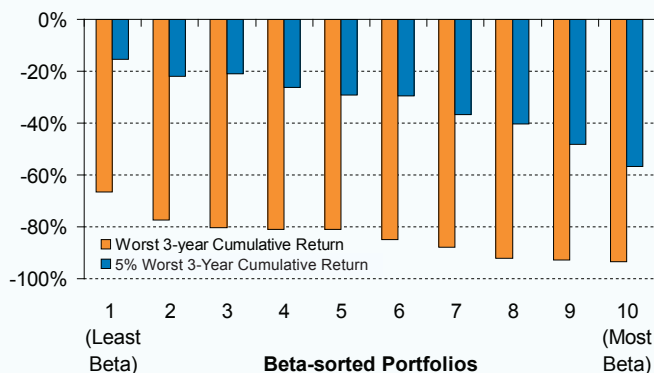
...And Smaller Equity Tails (Comparison of Worst 3-Year Cumulative Returns, 1927 – 2009)
