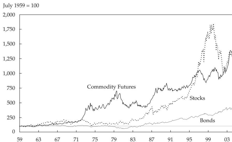
Figure 3. Inflation-Adjusted Performance of Stocks, Bonds, and Commodity Futures, July 1959–December 2004
